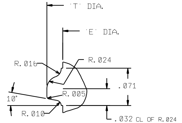
THREAD DETAIL SCALE 10:1 12 TPI
