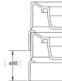
NESTING VIEW
