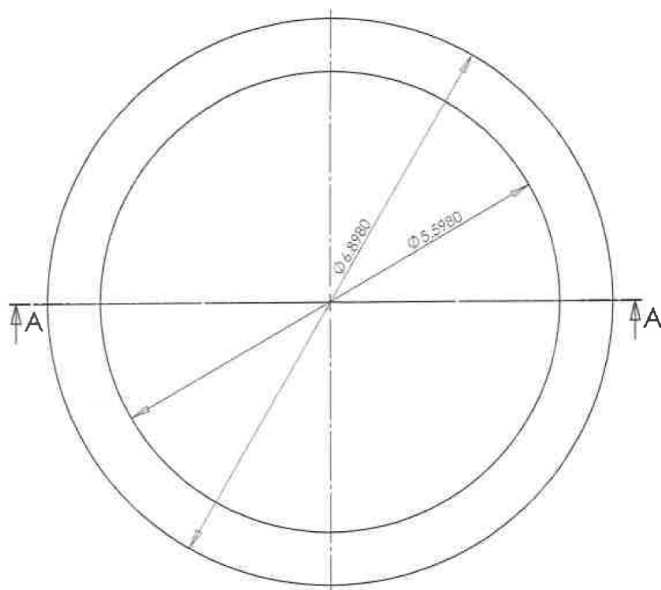
DETAIL B SCALE 5 : 1
