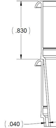
NESTING VIEW
