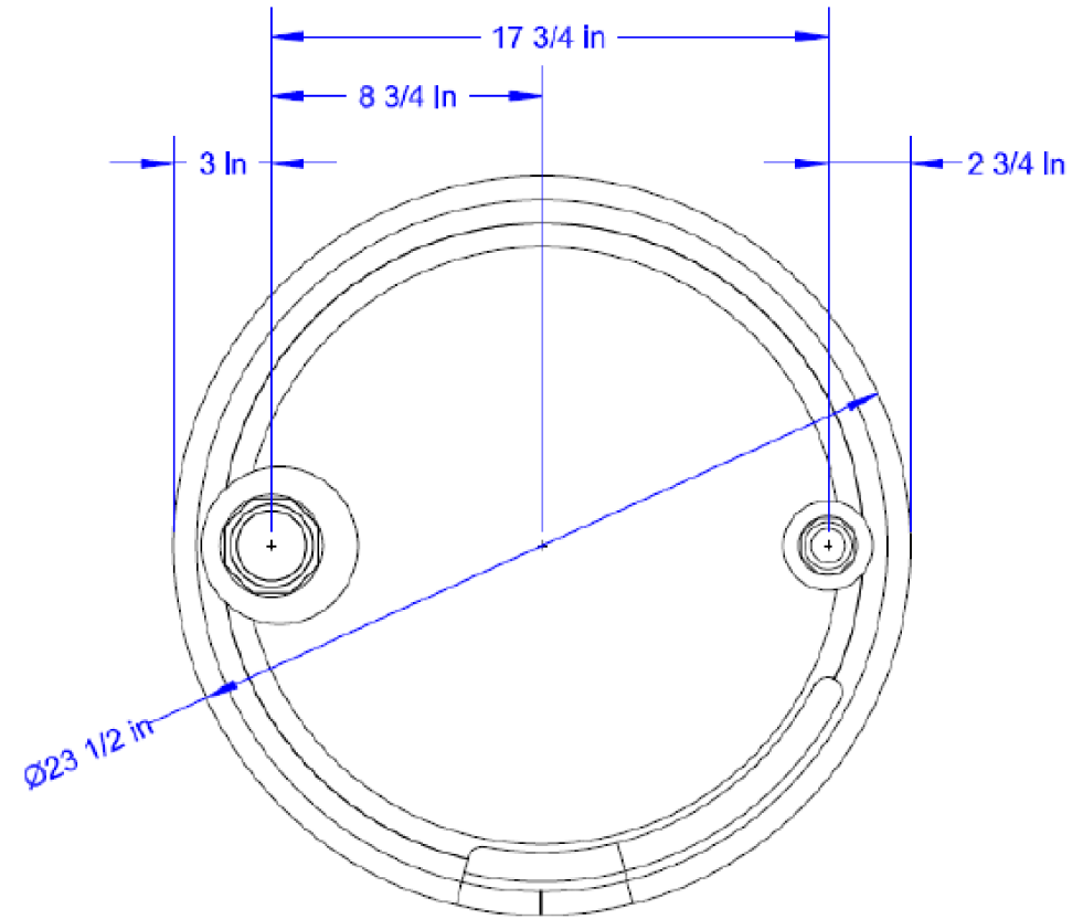
TOP VIEW
