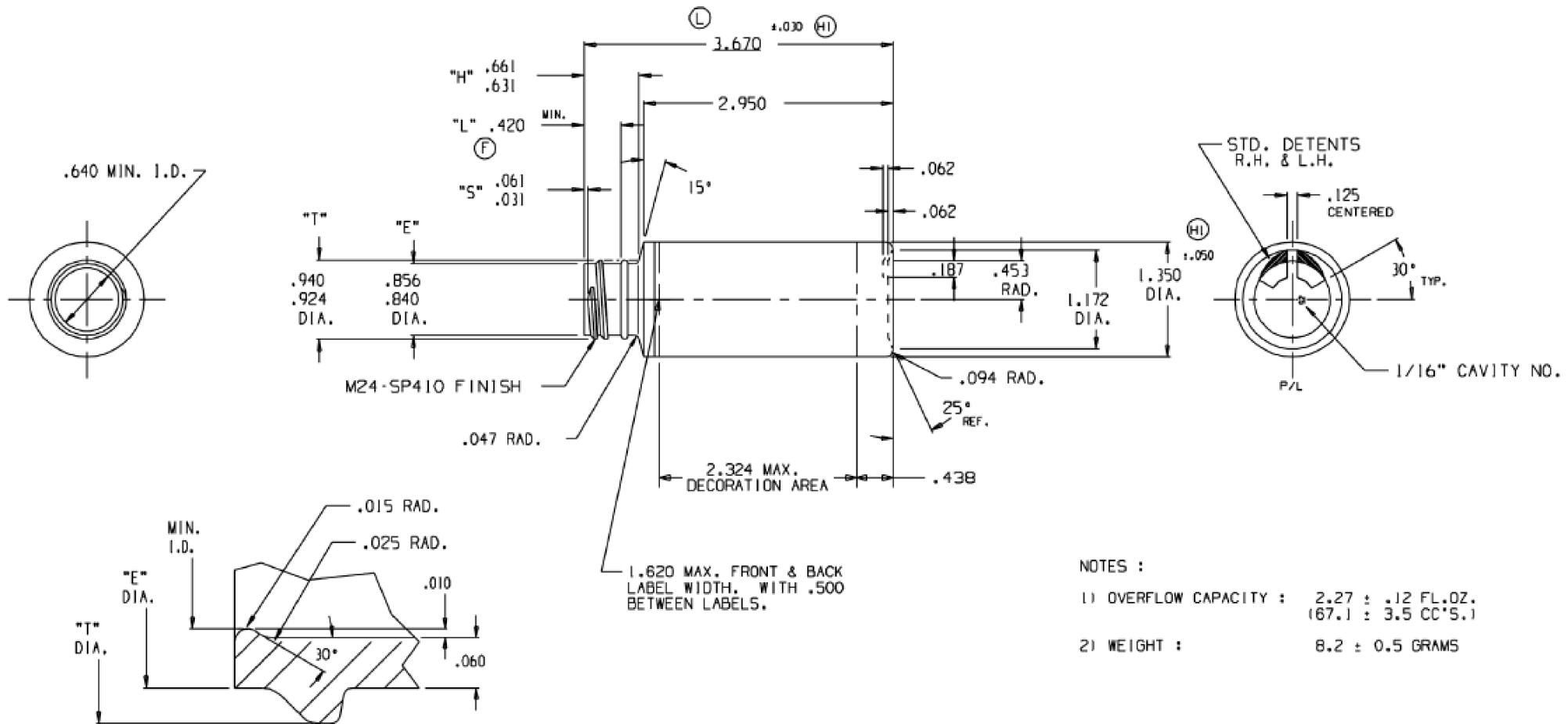
I.D. DETAIL
