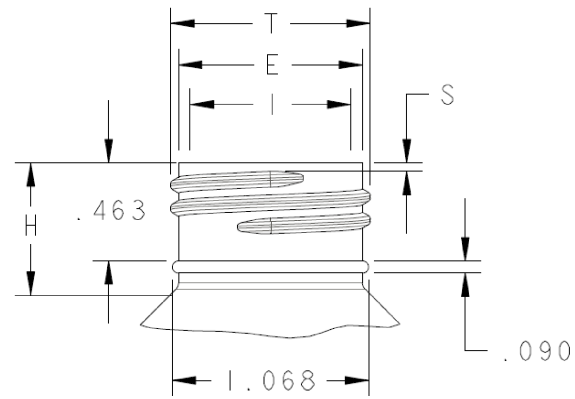
DETAIL A SCALE 3/2
