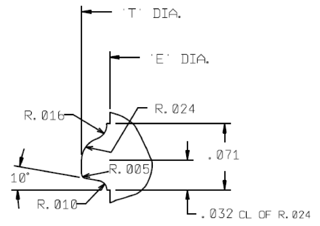
THREAD DETAIL SCALE 10:1 12 TPI
