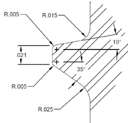
THREAD PROFILE SCALE 20:1
