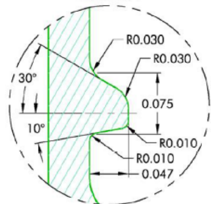
PLASTIC THREAD DETAIL SCALE 10 : 1
