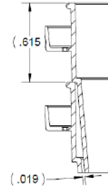
NESTING VIEW
