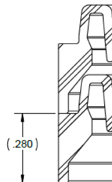
NESTING VIEW
