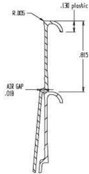
VIEW SHOWING AIR GAP SCALE 5.000
