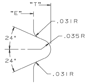
TYPE "B" THREAD DETAIL SCALE 10 X 1
