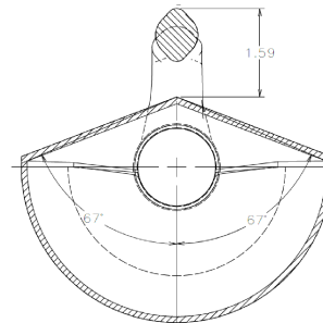
SECTION B-B SCALE 3:4
