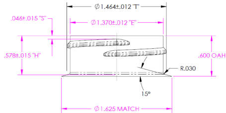
38mm SP400 NECK DETAIL 2X SCALE "M" STYLE THREAD ONE FULL TURN 6 THREADS PER INCH
