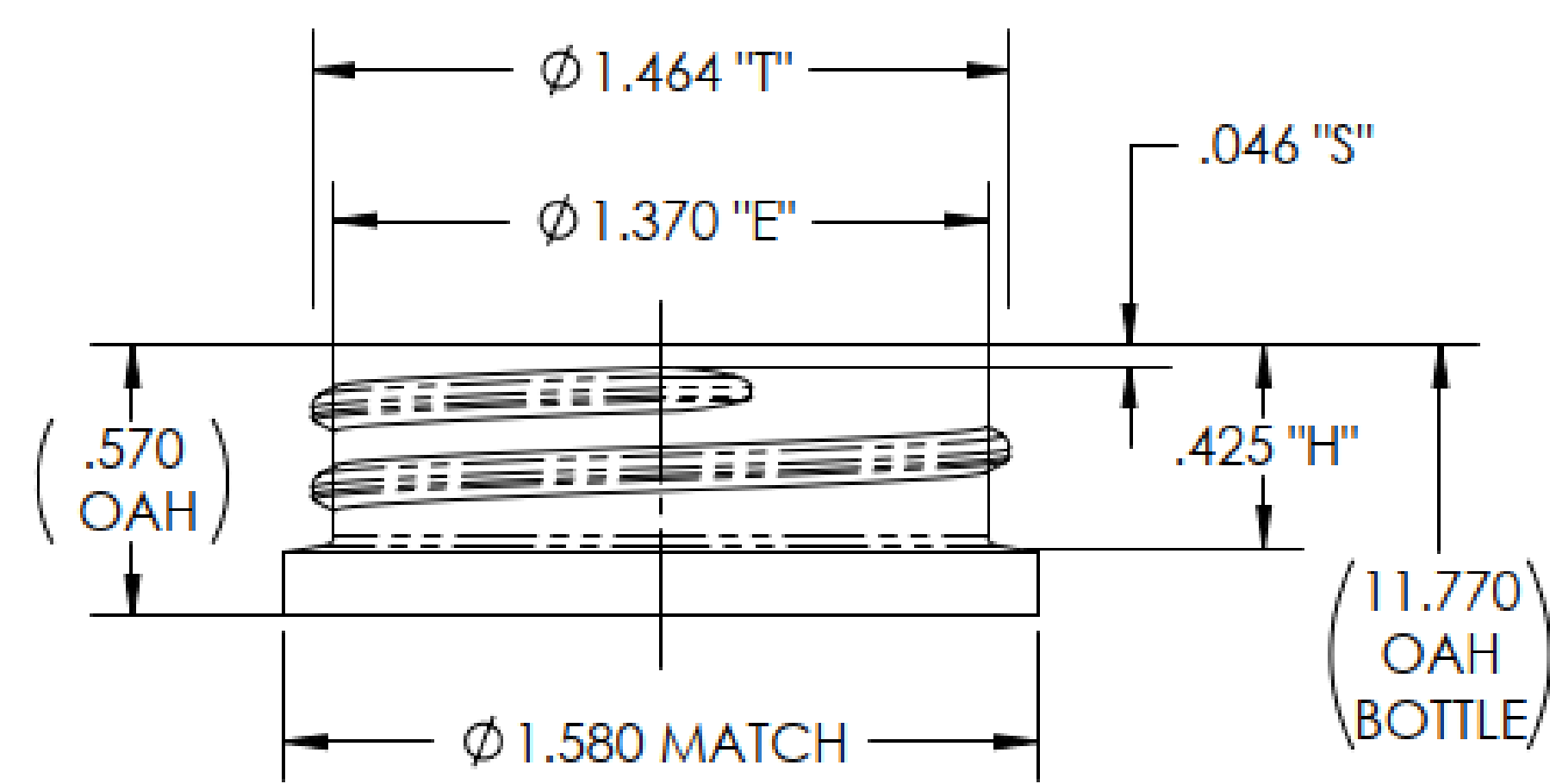
38mm SP-400 NECK FINISH DETAIL 3:2X SCALE
