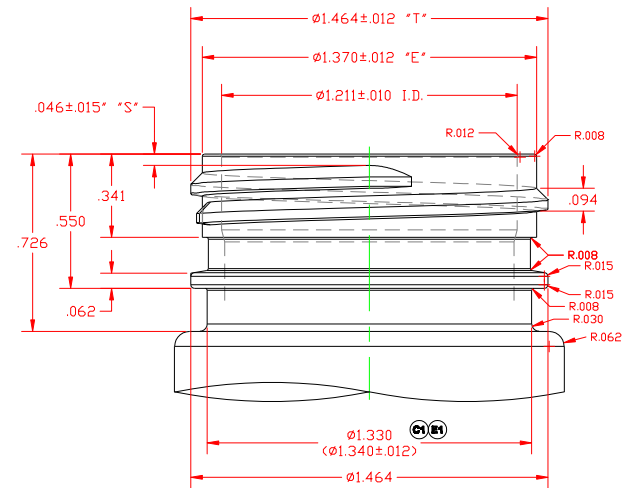
NECK FINISH DETAIL SHOWN 4x SCALE
