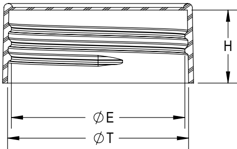
SECTION H-H
