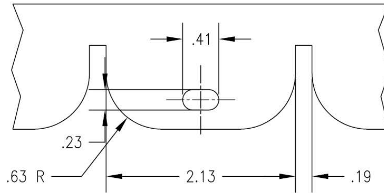
VIEW OF LUG (16) REQ'D. TYP.
