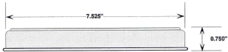
COVER SIDE VIEW
