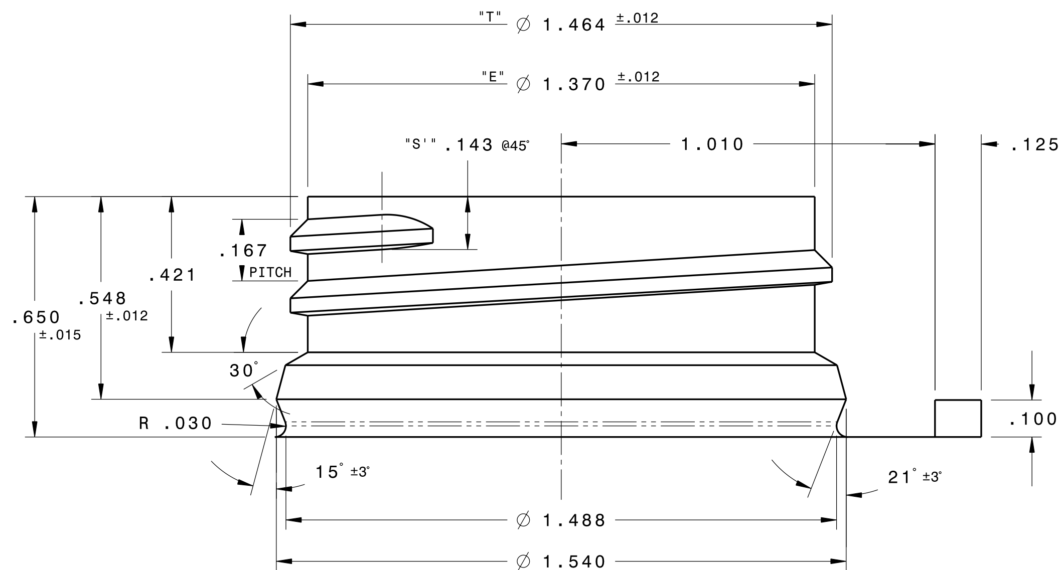
38 CR SNAP LOK FINISH DETAIL SCALE 3X 6 T.P.I. 1-1/2 TURNS FULL THREAD REF: SUNBEAM DWG M-2033-6
