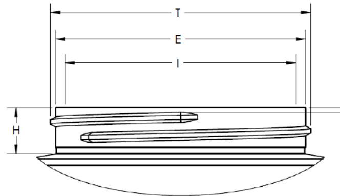
DETAIL A SCALE 1.5 : 1
