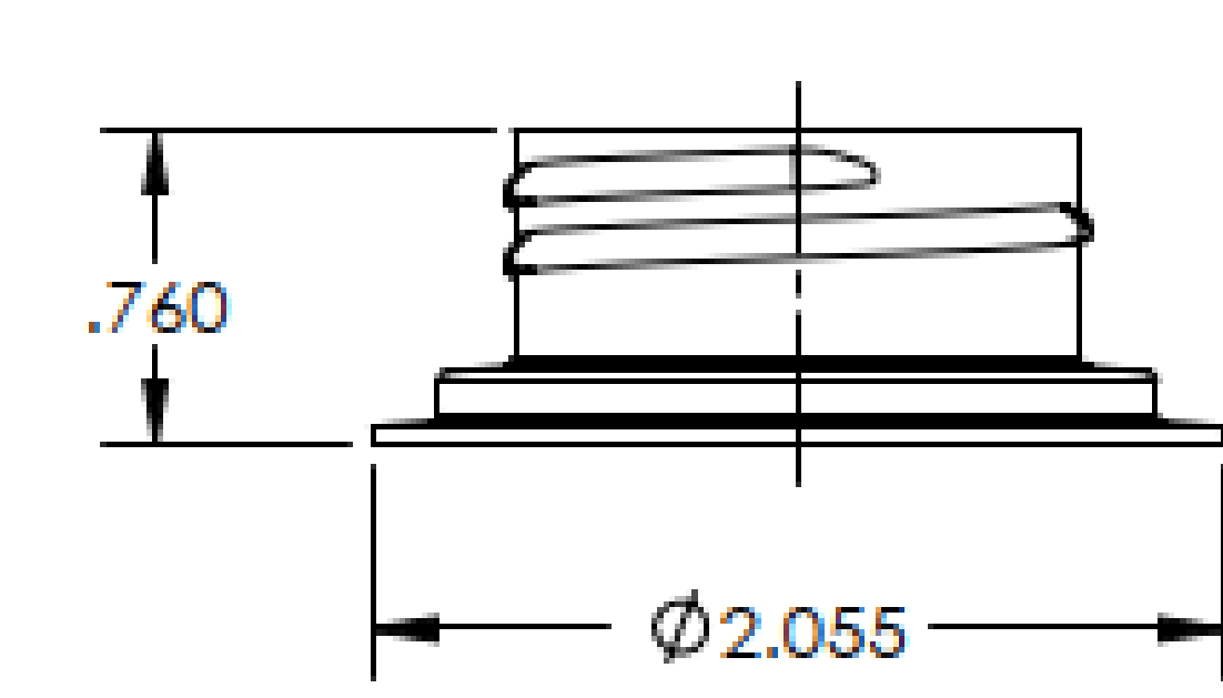
Ⓕ 38mm SP-400 SCREW FINISH "M" STYLE THREAD WITH 1-1/2 TURNS
