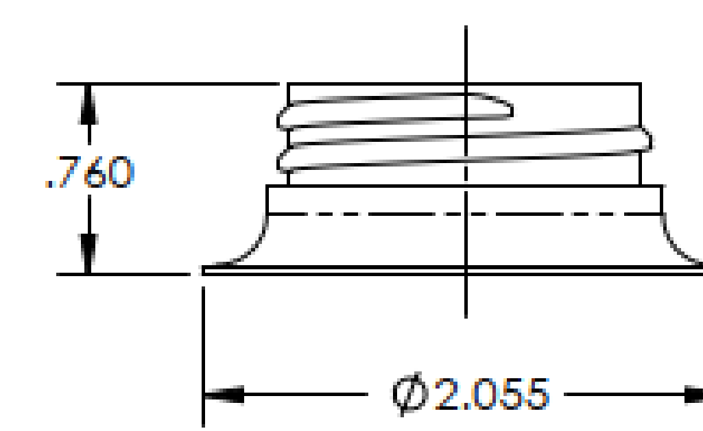
Ⓔ 38mm SP-400 SCREW FINISH "M" STYLE THREAD WITH 1-1/2 TURNS
