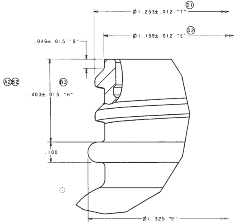
FINISH DETAIL SCALE 8:1
