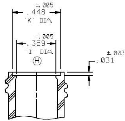
NECK DETAIL SCALE 2:1
