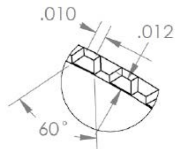
120 KNURLS DETAIL B SCALE 10 : 1
