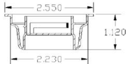
SPOUT DIMENSIONS
