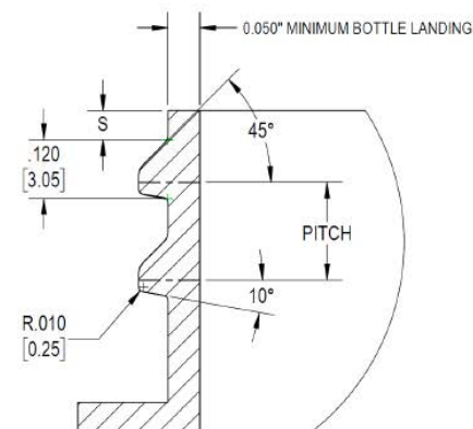
DETAIL E SCALE 4 : 1
