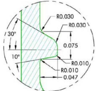
PLASTIC THREAD DETAIL SCALE 10 : 1
