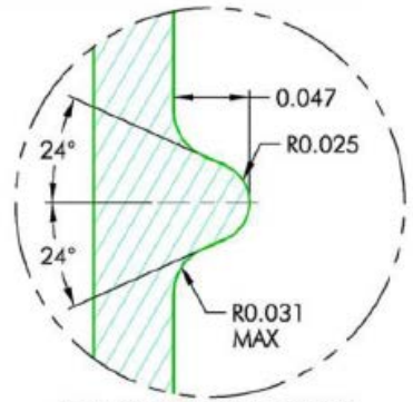
GLASS THREAD DETAIL SCALE 10 : 1
