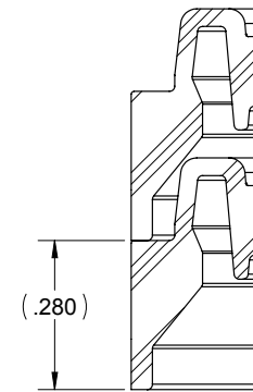
NESTING VIEW
