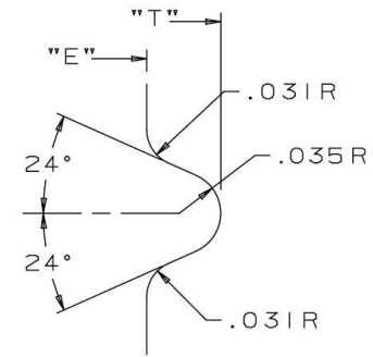
TYPE "B" THREAD DETAIL SCALE 10 X 1
