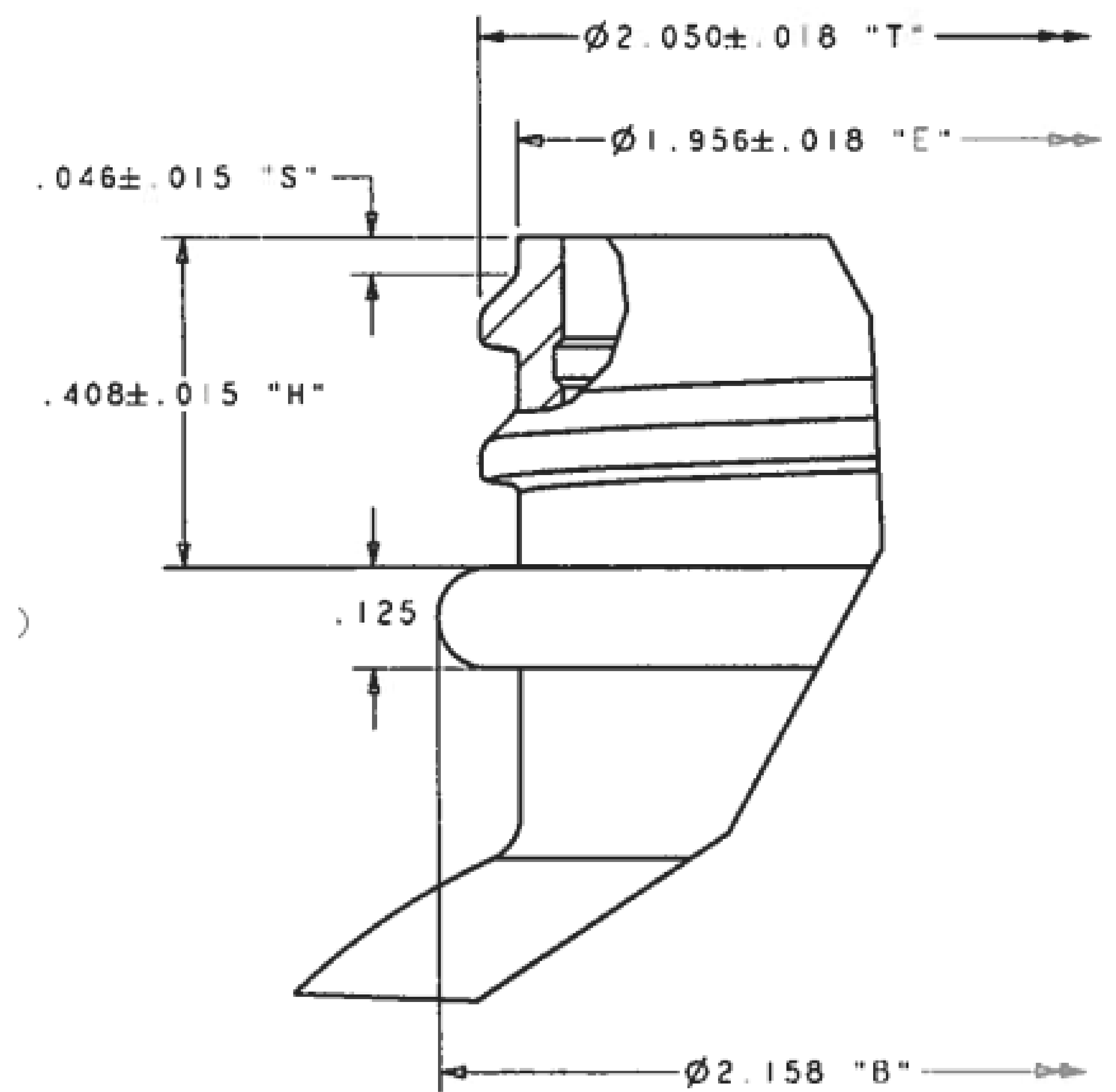
FINISH DETAIL SCALE 5:1
