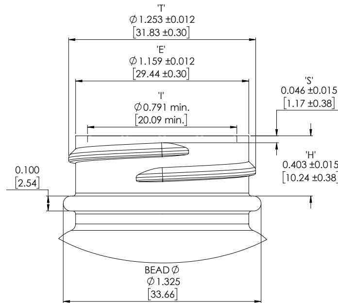
DETAIL A SCALE 3 : 1 NECK DETAIL 33-400 STANDARD NECK FINISH MIN. 1 TURN OF 'M' STYLE THREAD 6 T.P.I.
